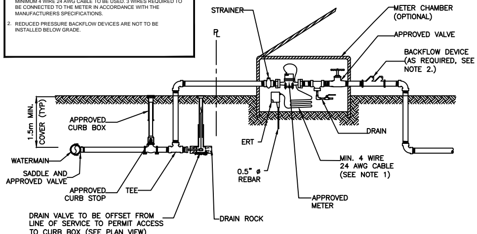
SECTION VIEW
