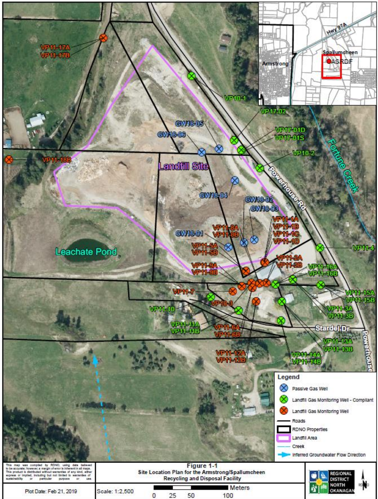
FIGURE 1 - Site Map of Landfill Gas Monitoring Wells in 2022
